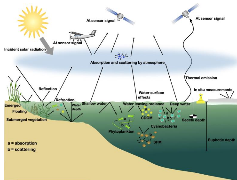
Figure 5. Interaction between radiation, remote sensing indicators of lake ecology and sensors (according Dörnhöfer & Oppelt, 2016).
